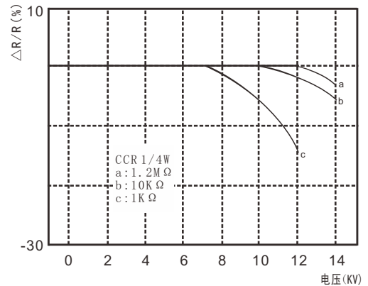
CCR 1/4W电涌试验 (Surge test)
