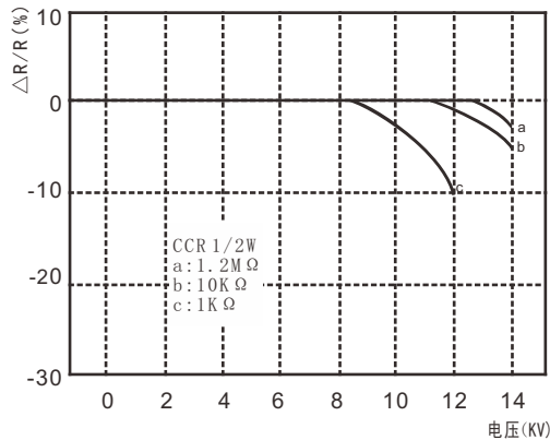
CCR 1/2W电涌试验 (Surge test)
